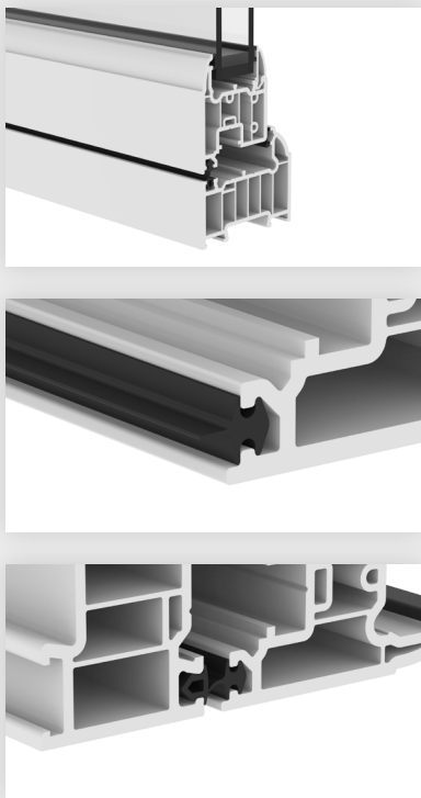
LGA413 Flush Sash Gasket
